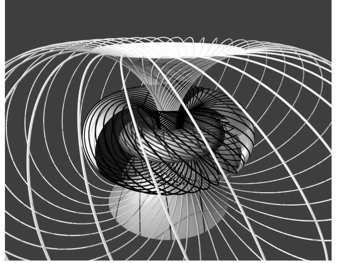
Figure 4. Stereographic projection of surfaces of constant coordinate x_3 for x_3 = \pi/8, \pi/4, 3\pi/8 . The circles are geodesics - coordinate lines of x_1 . Each circle represents one fiber of the ‘‘Hopf fibration’’ S^3 \rightarrow S^2 . For more details, as well as for the relation to quantum spin 1/2 states see Ref. [30, p. 60-68]
