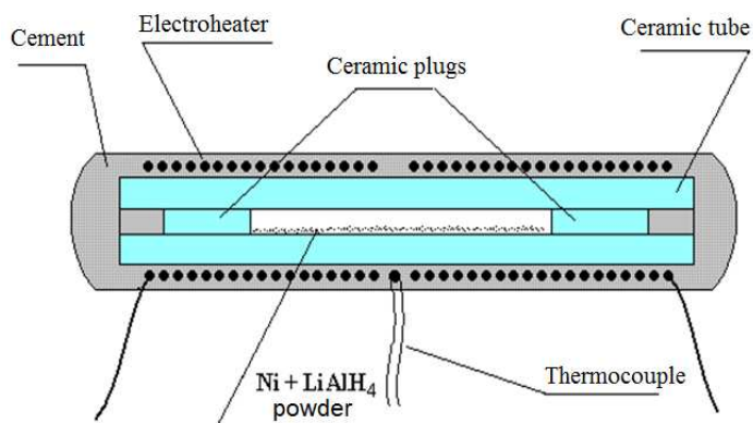
Figure 1. (Right) scheme of the device and (left) the picture of the reactor before operation.
